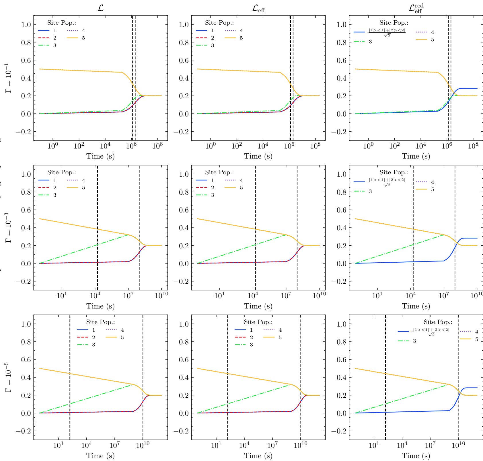
Time Evolution of Site Populations under \mathcal{L} , \mathcal{L}_{\text{eff}} , and \mathcal{L}_{\text{eff}}^{\text{red}} Initially: Site 4 and 5 at 0.5, rest empty N=5 ; J = 10^{-1} ; \epsilon = 10^{-4}
